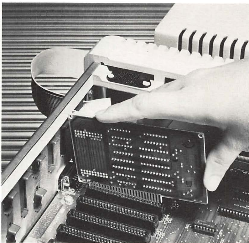
Figure 4-3. Install the Controller Card
