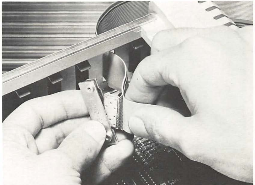
Figure 2-5. Place the Clamp Over the Metal Flap
