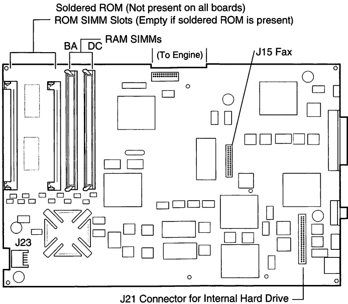
Figure 10. LaserWriter 16/600 PS I/O Controller Board
