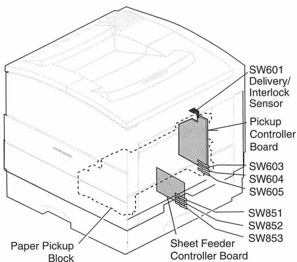
Figure 25. Sensing Switches
