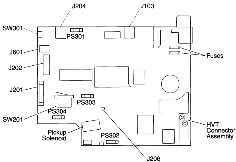
Figure 48. Personal LaserWriter 320 Controller Assembly Board
