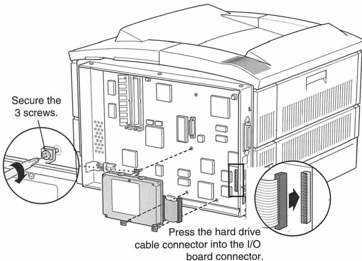
Figure 18. Installing the Internal Hard Drive
