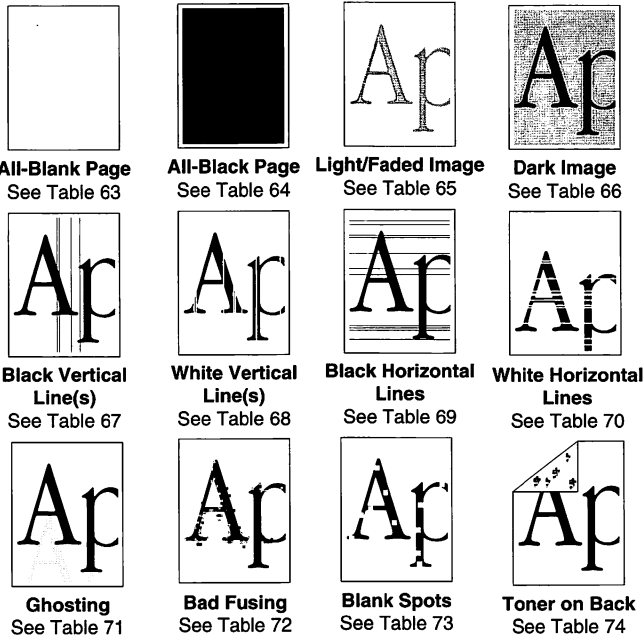
Figure 44. Print Quality Problems
