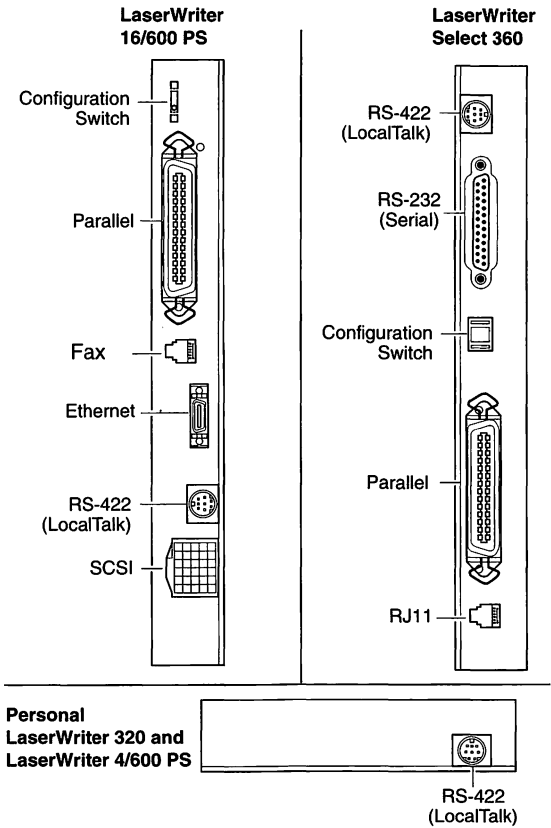
Figure 5. Printer Ports
