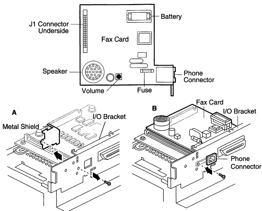
Figure 39. LaserWriter Select 360 Fax Card Upgrade
