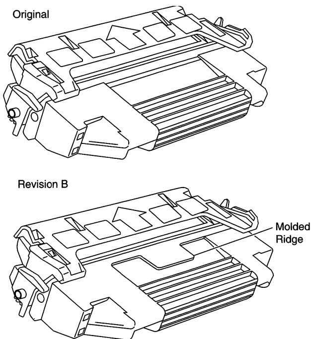
Figure 23. Comparison of LaserWriter Pro 600/630 Toner Cartridges
