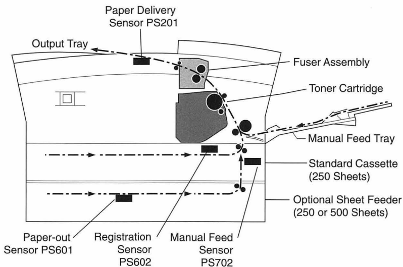
Figure 41. Paper Sensors and Paper Path Locator
