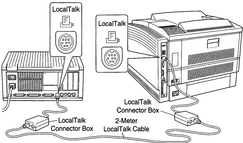
Figure 1. LocalTalk Connection
