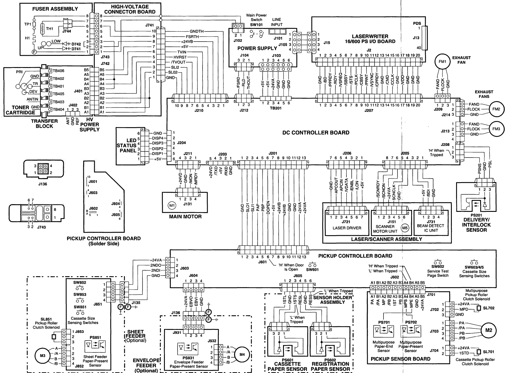
Figure 30. LaserWriter 16/600 PS Wiring Diagram
