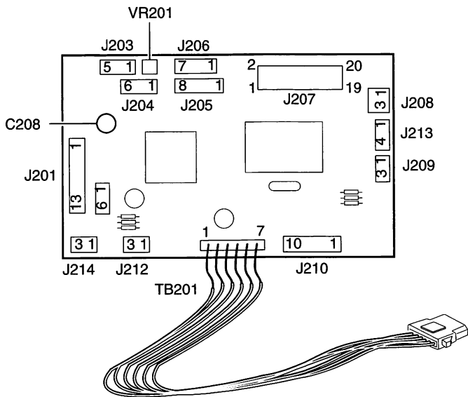
Figure 11. LaserWriter 16/600 PS DC Controller Board
