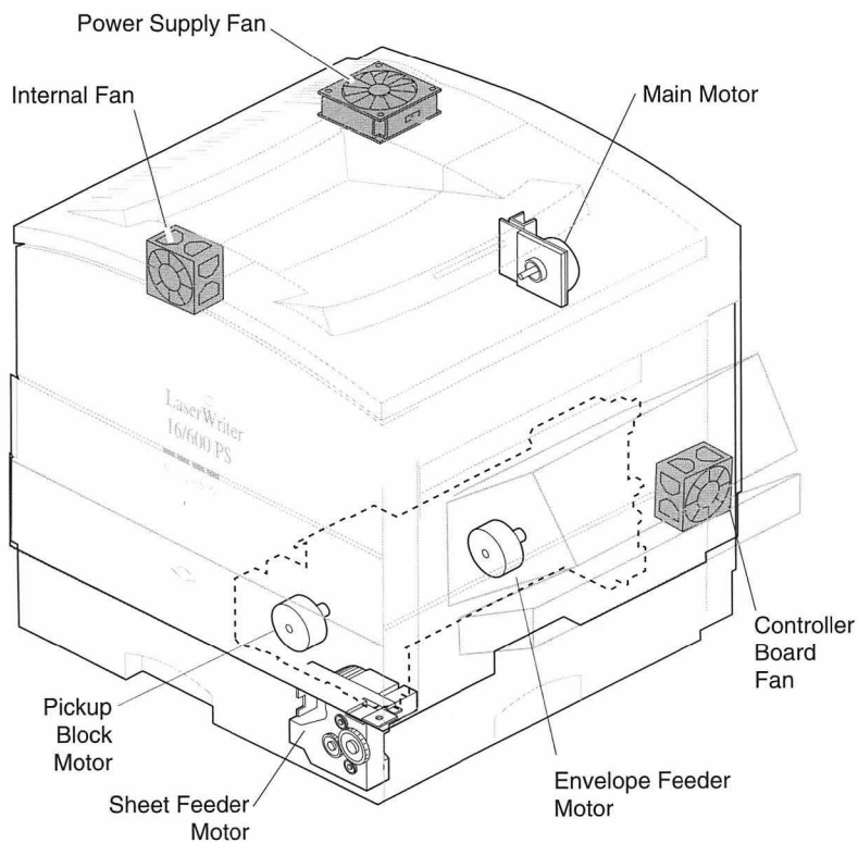
Figure 26. Paper Path, Motors, and Fan Locations
