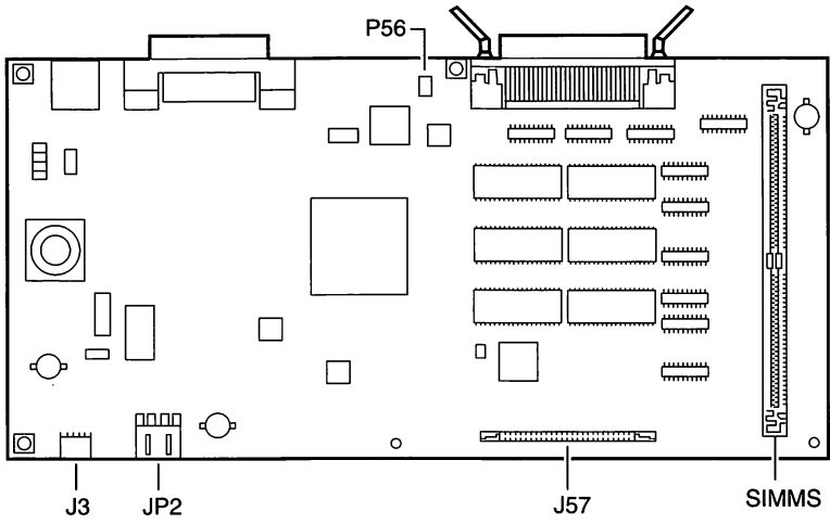
Figure 32. LaserWriter Select 360 I/O Controller Board
