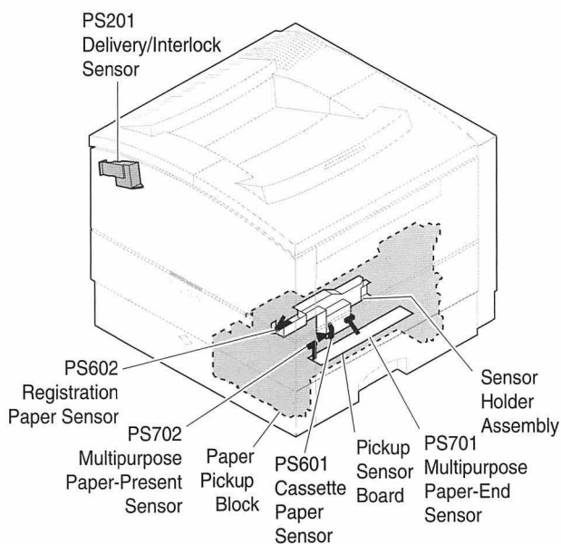
Figure 24. Paper Sensors
