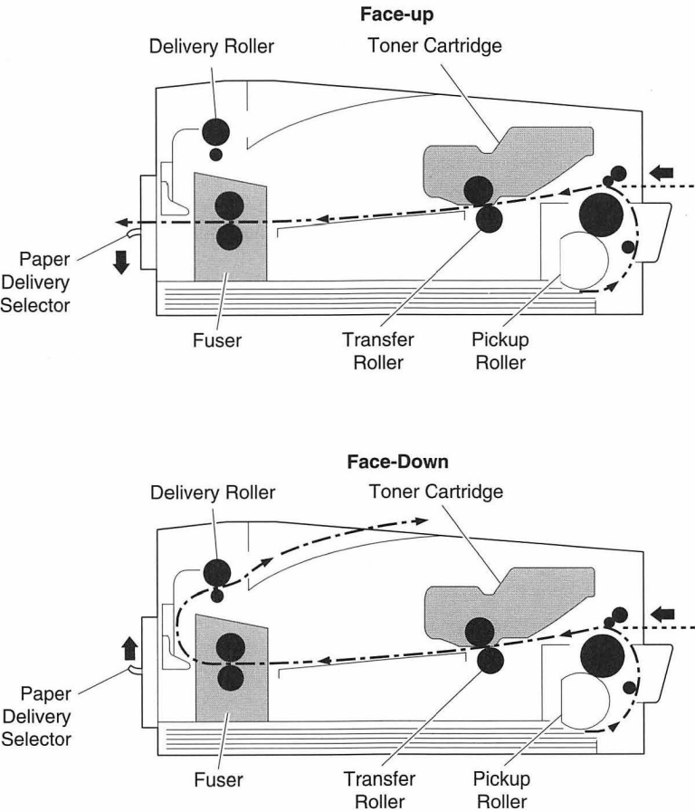
Figure 51. Paper Paths
