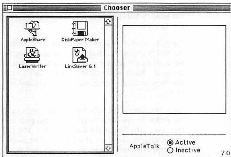
Figure 8 Chooser window.
