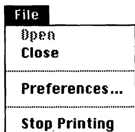
Figure 18 PrintMonitor menu.
