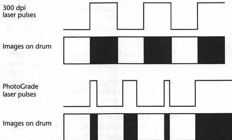
Figure 7 PhotoGrade laser pulse control.
