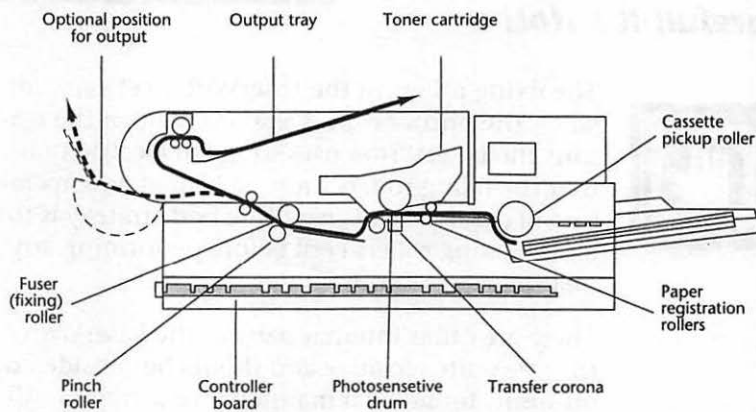
Figure 27 LaserWriter internal view (side).
