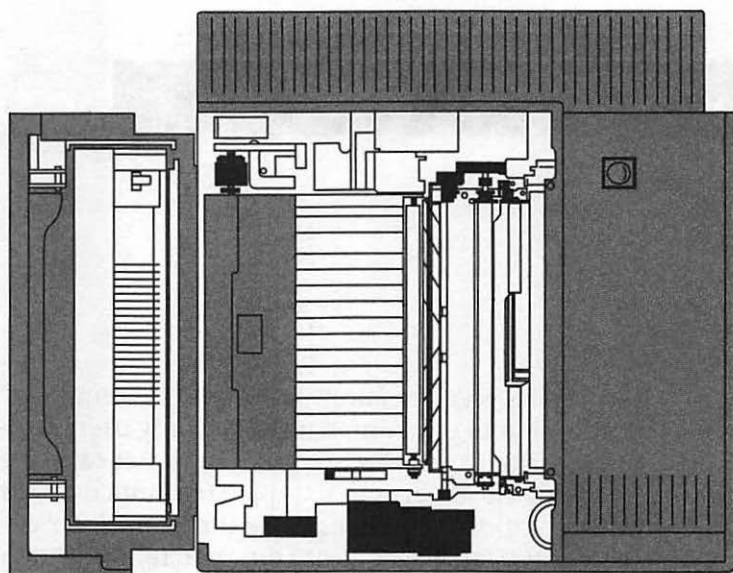
Figure 26 LaserWriter internal view (top).
