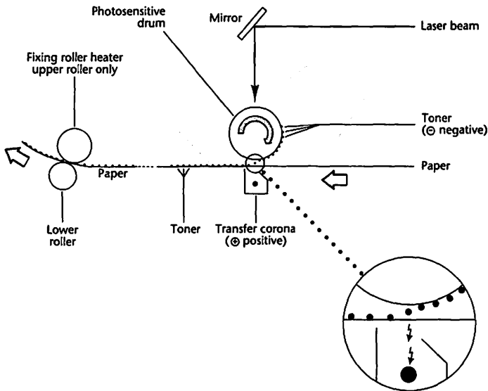
Figure 1 LaserWriter II paper path.
